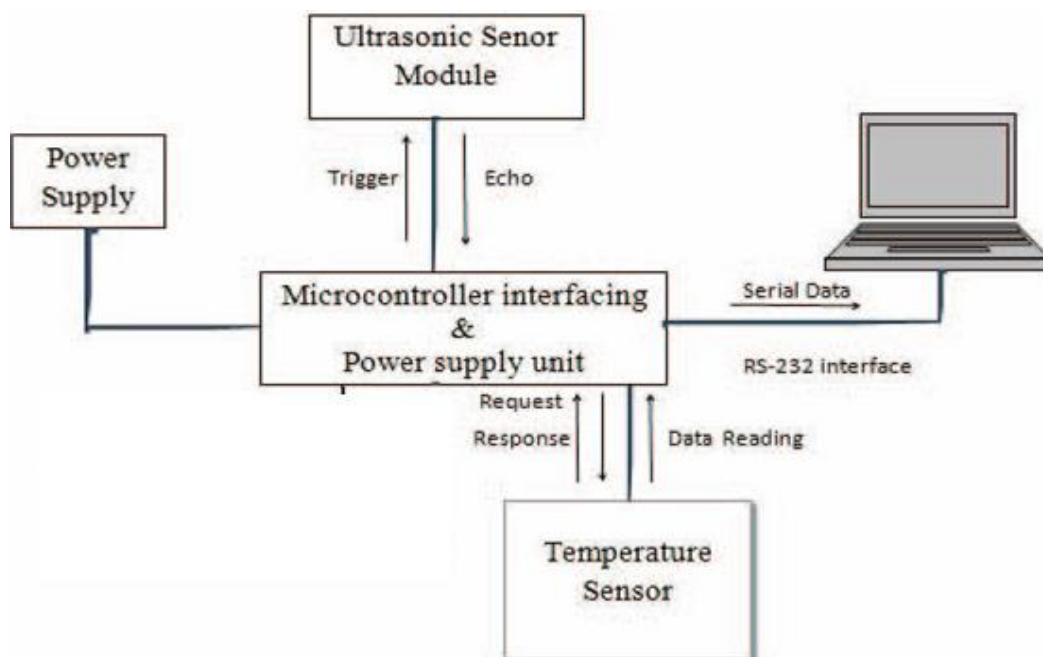
Fig 4.1. Block diagram of system
