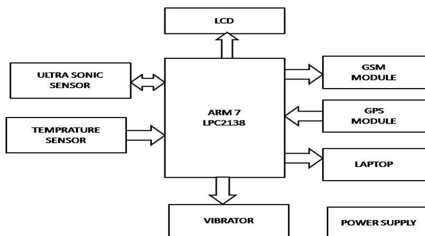
Fig. 5.2 Hardware Block Diagram
